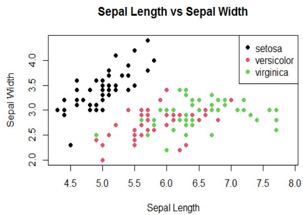
Fig 3 – Scatterplot of sepal length and sepal width of all three species
