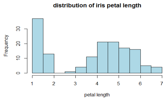
Fig 1—Histogram of petal length
