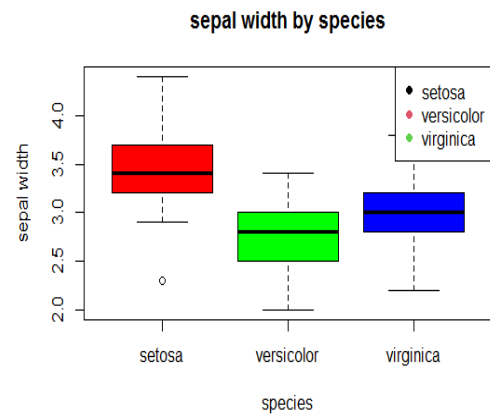
Fig 2 – Boxplot of sepal width
